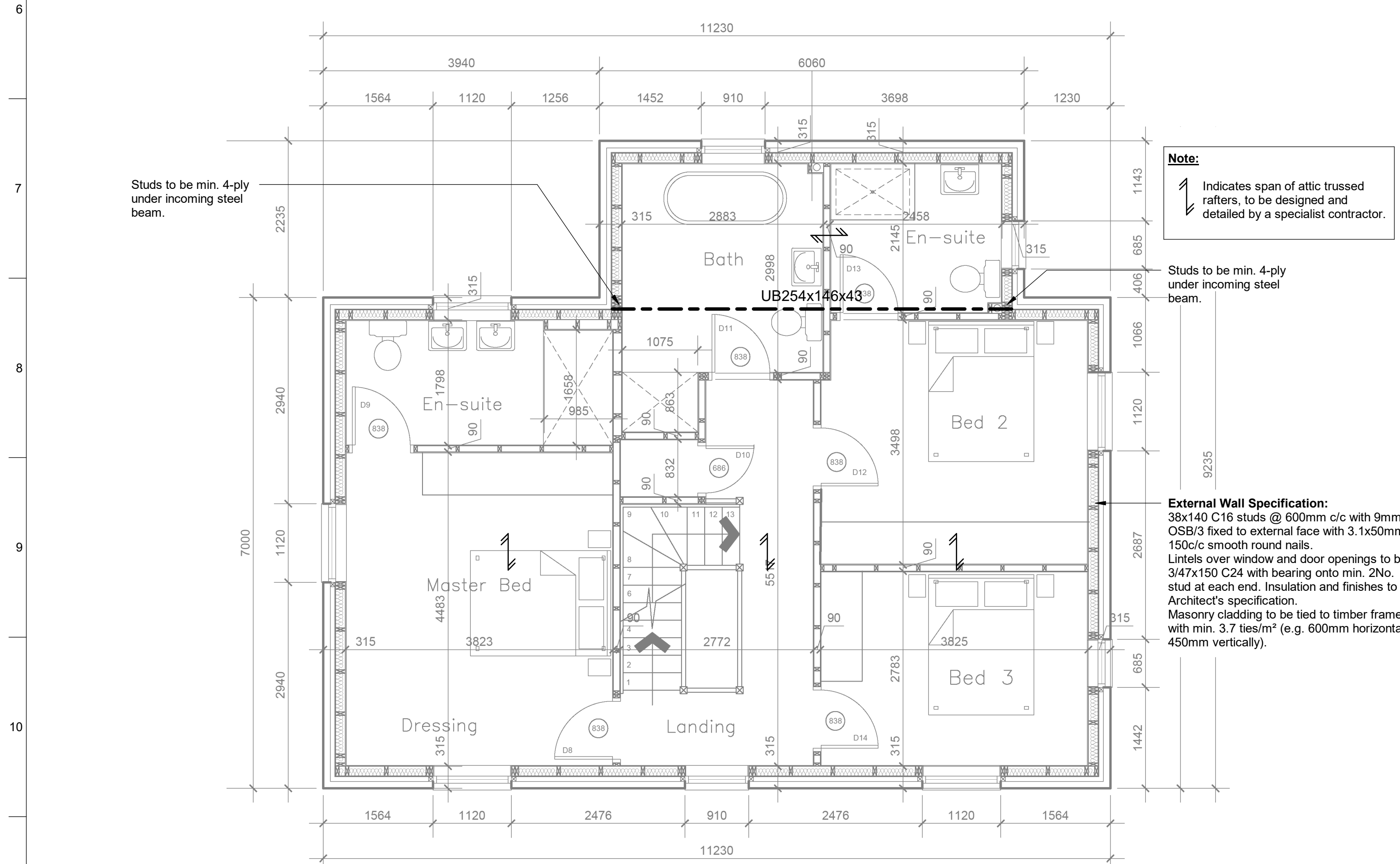
Plot 3 - First Floor Plan 1 : 50
