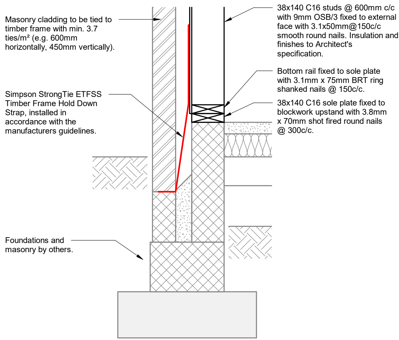
Plot 3 - Holding Down Strap Detail 1 : 10
