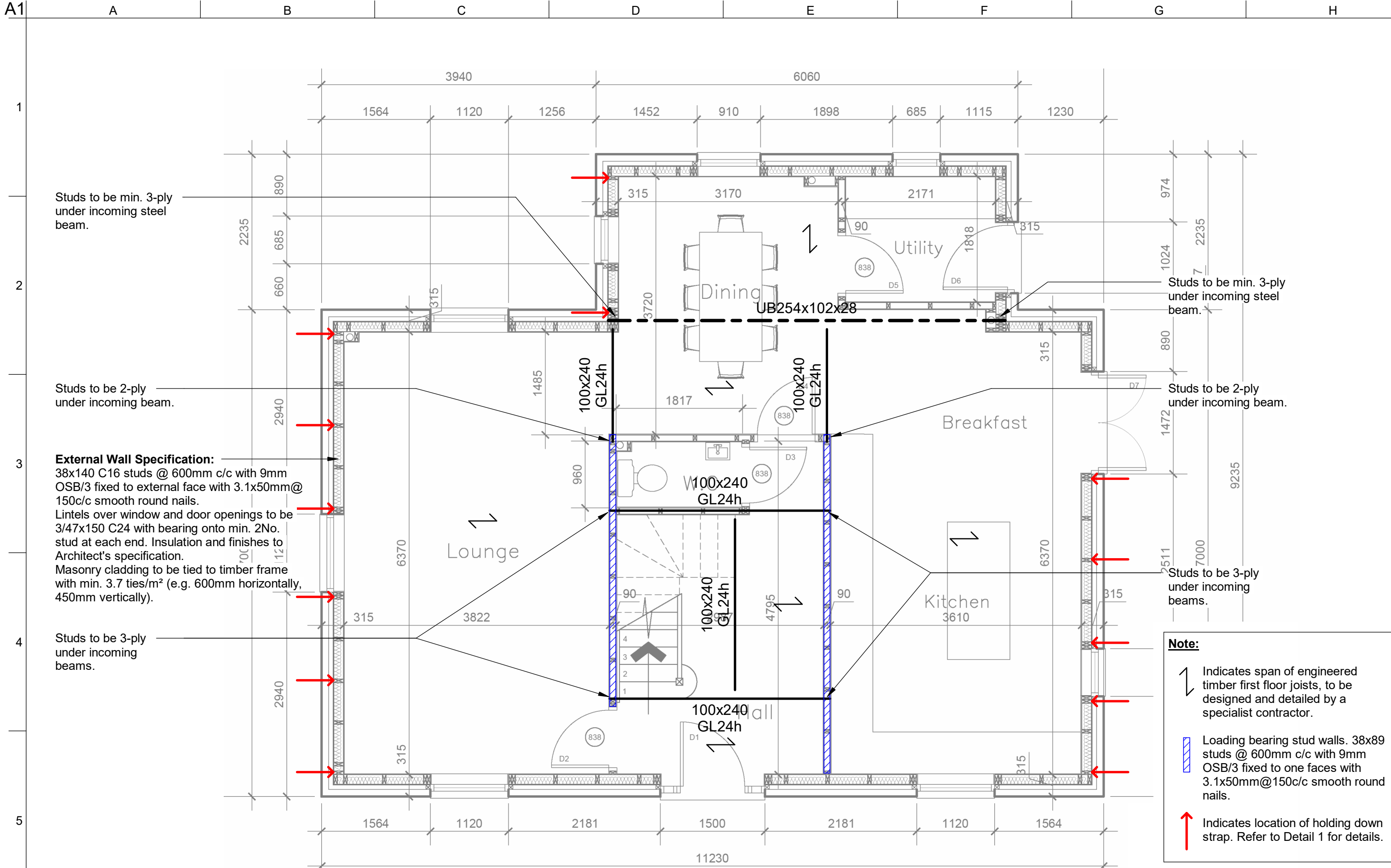
Plot 3 - Ground Floor Plan 1 : 50
